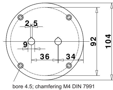
tpac105 - for the input of 6 mm pole terminals
