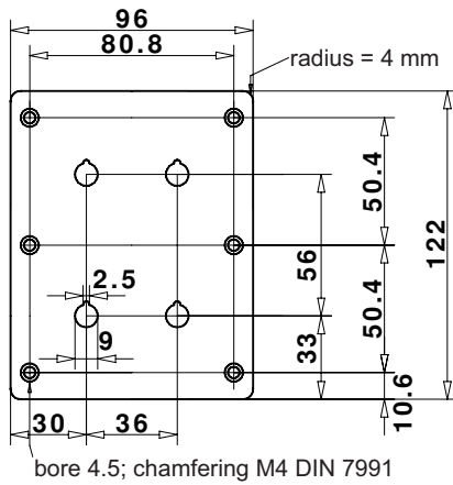
tpac122 - for the input of 6 mm pole terminals
