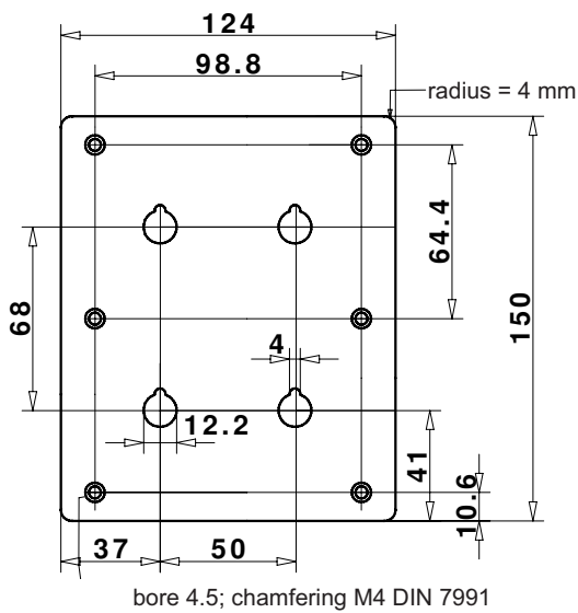
tpac150 - for the input of 8 mm pole terminals
